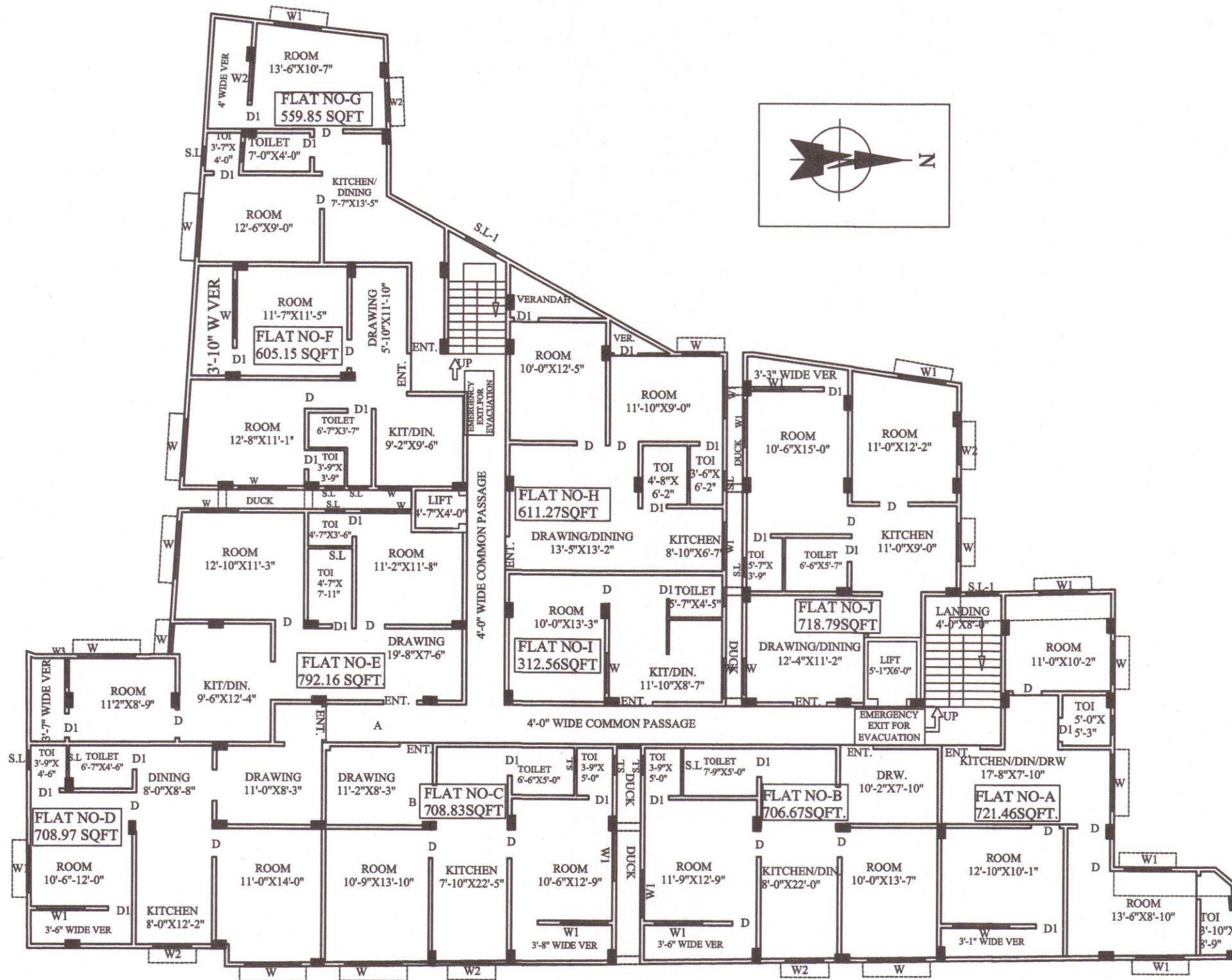
PROPOSED 5TH FLOOR PLAN SCALE 1:96
